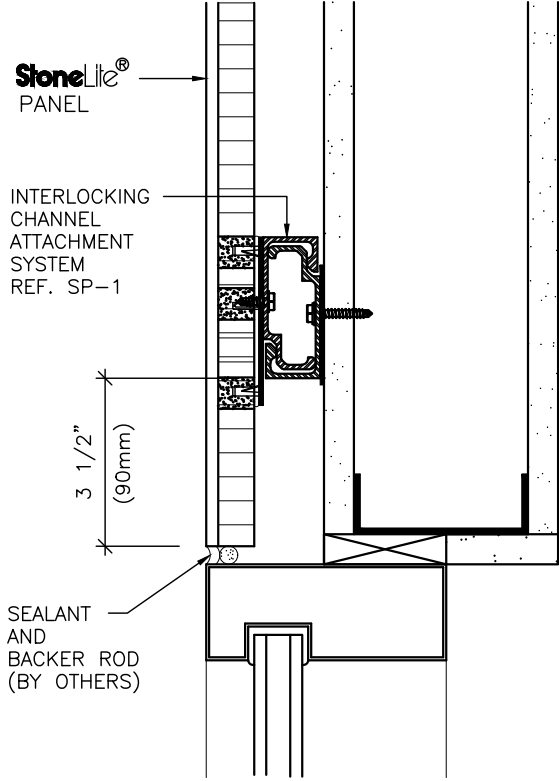
FLUSH WINDOW HEAD
