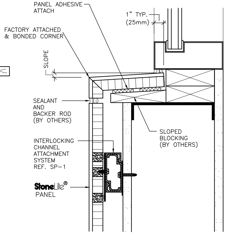
RECESSED WINDOW SILL
