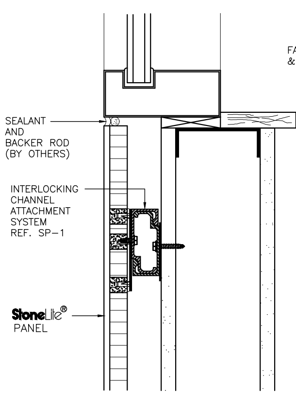
FLUSH WINDOW SILL
