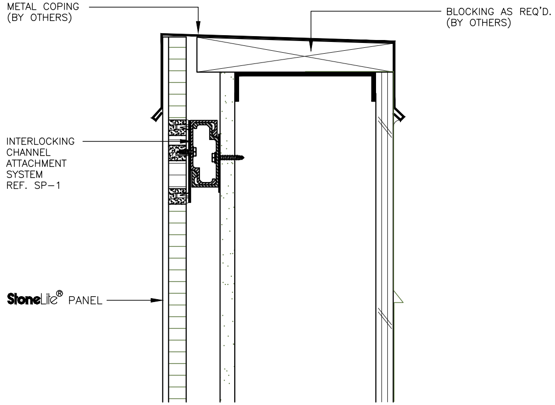
TYPICAL COPING DETAIL
