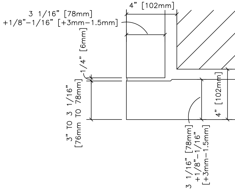
BUTT CORNER 3 1/16" +1/8"-1/16" [78mm +3mm-1.5mm]
