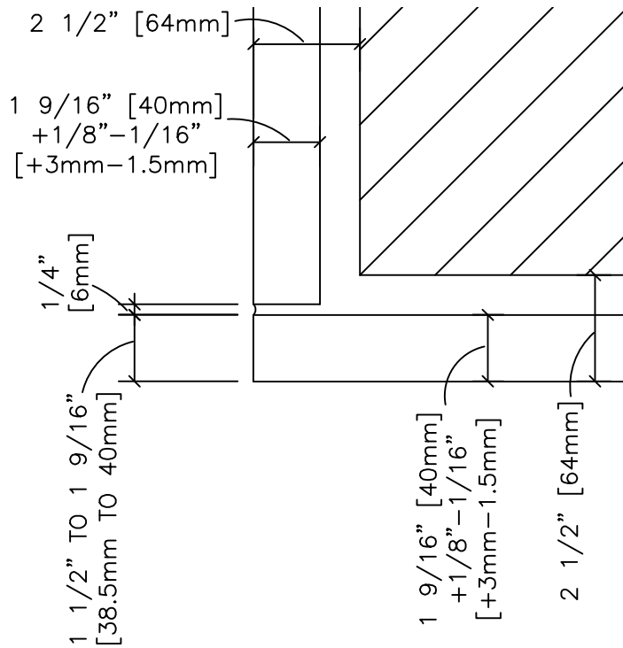
BUTT CORNER 1 9/16" +1/8"-1/16" [40mm +3mm-1.5mm]
