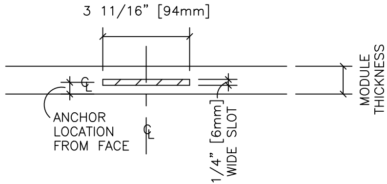
TOP VIEW - 1/4" [6mm] WIDE ANCHOR SLOT
