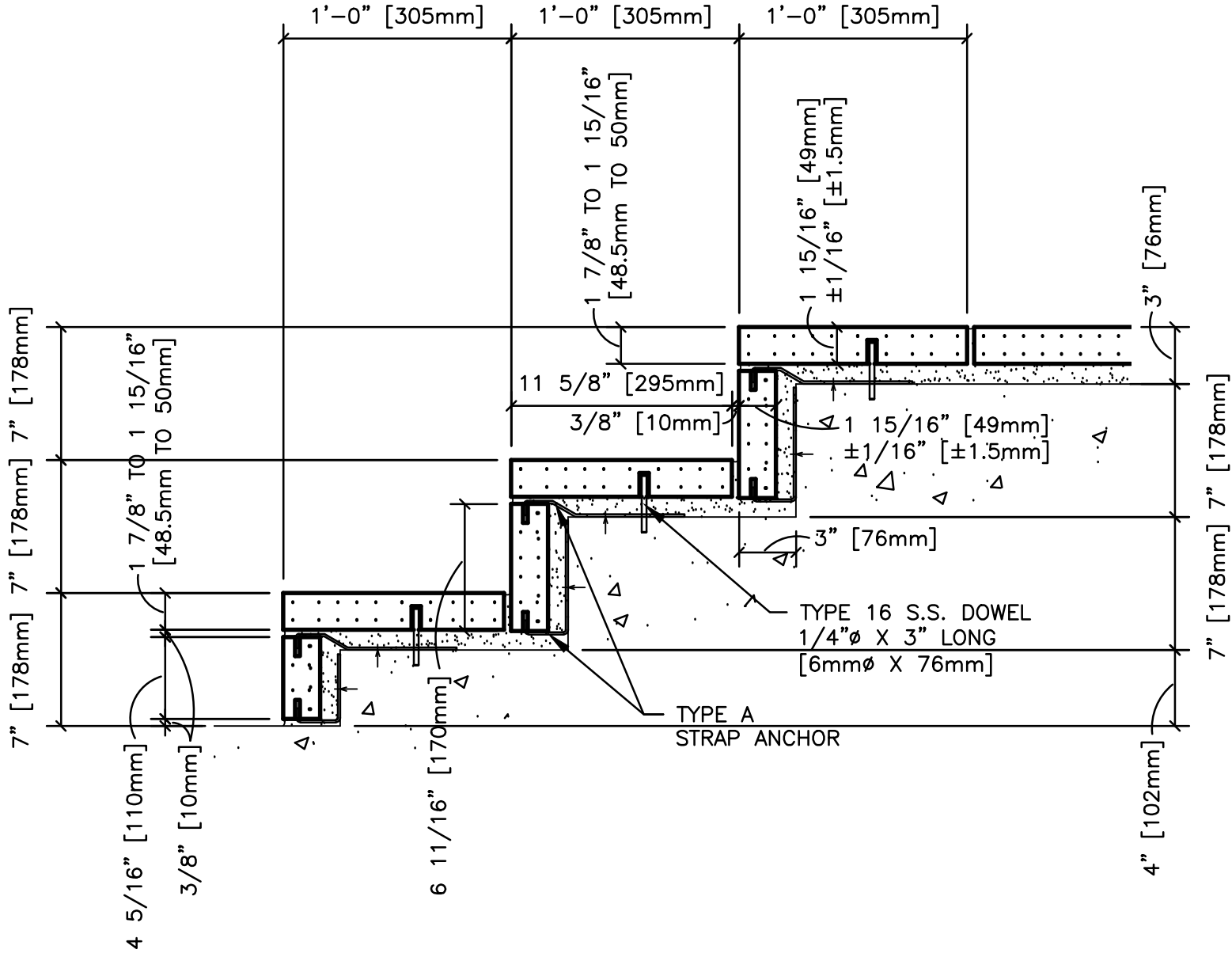
VENEERED TREAD AND RISER
