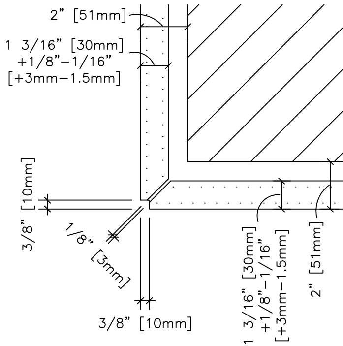
3/8" X 3/8" QUIRK MITER CORNER WITH 1/8" JOINT
