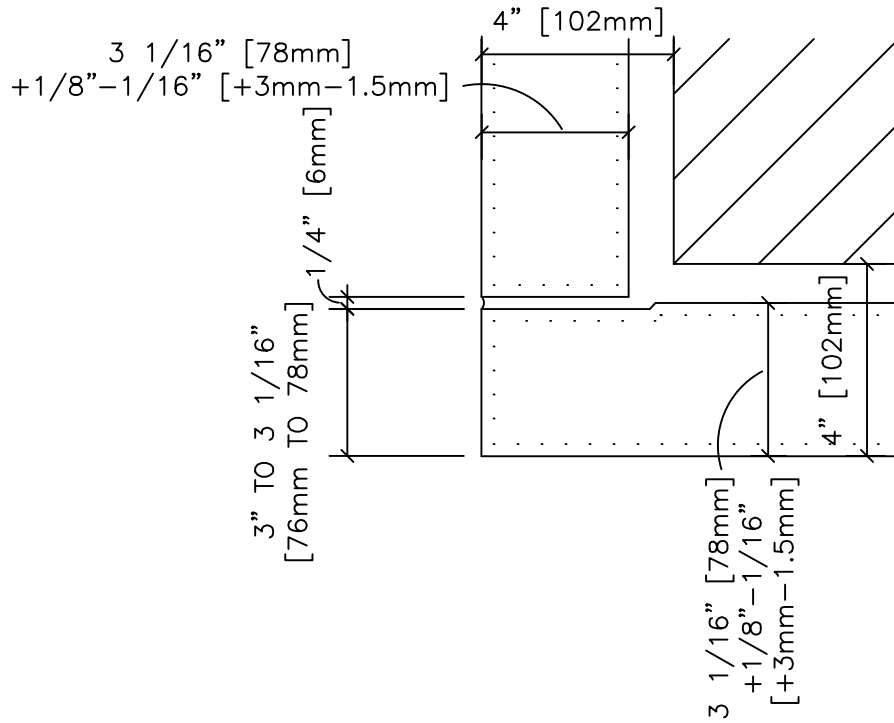
BUTT CORNER 3 \frac{1}{16}'' +1/8''-1/16'' [78mm +3mm-1.5mm]
