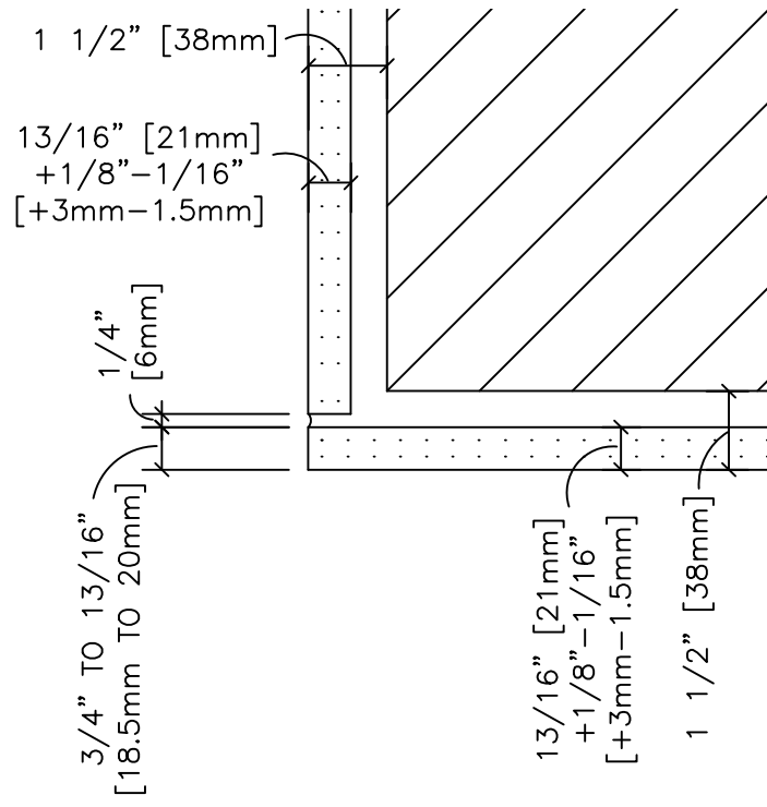
BUTT CORNER 13/16" +1/8"-1/16" [20mm +3mm-1.5mm]
