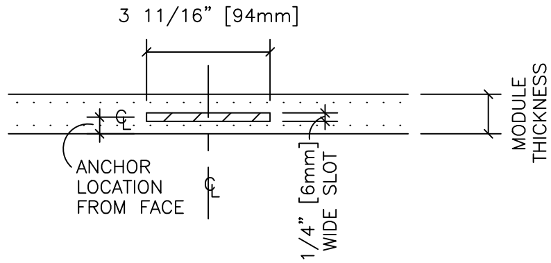
TOP VIEW - 1/4" [6mm] WIDE ANCHOR SLOT
